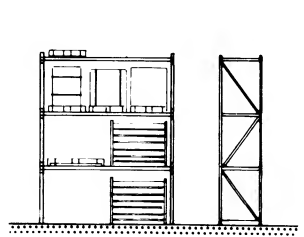
⑭ Pallet racks of prefabricated components (longitudinal transverse shelving)
